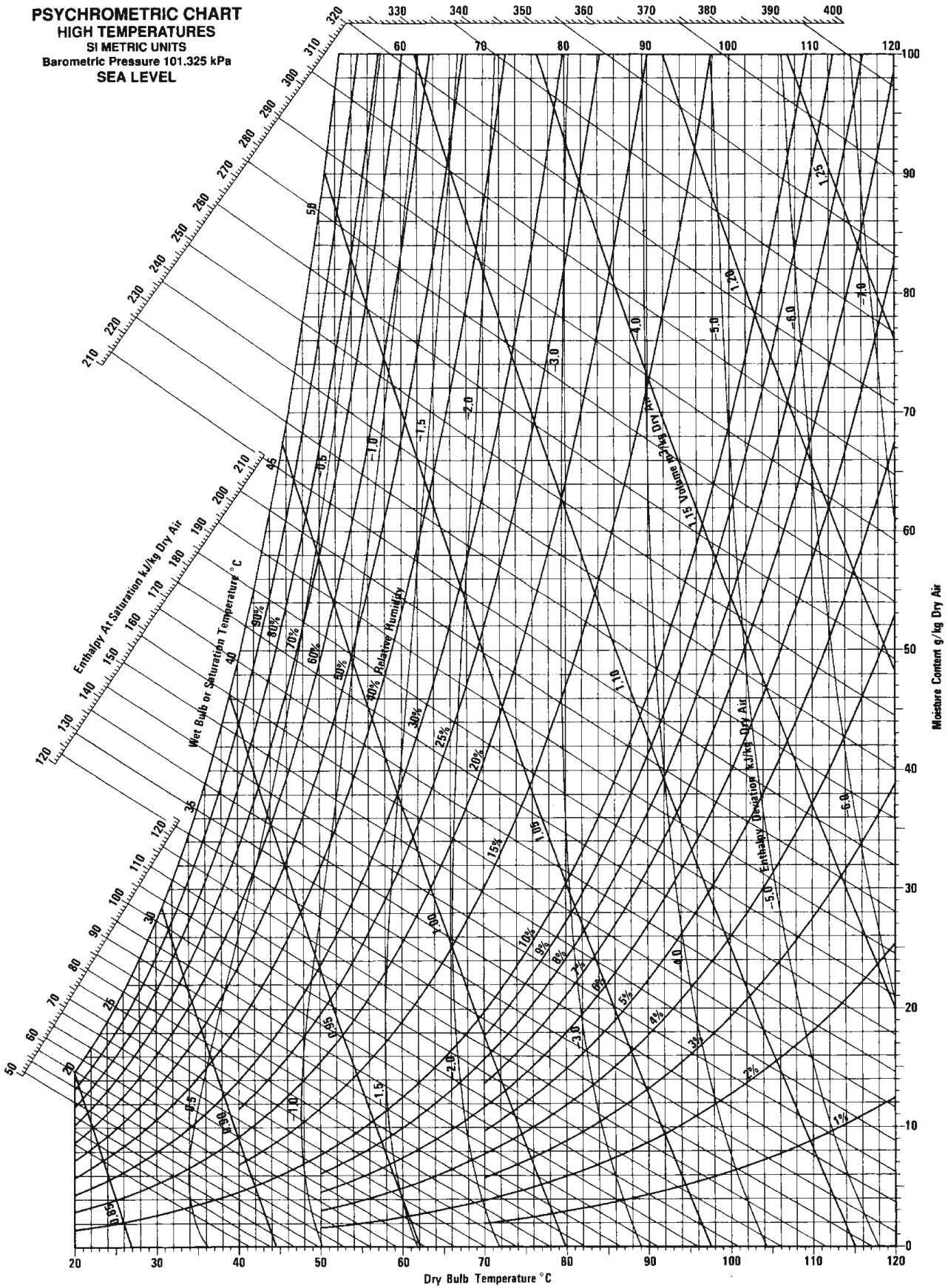
■ Figure A.5.1 Psychrometric chart for high temperatures.
